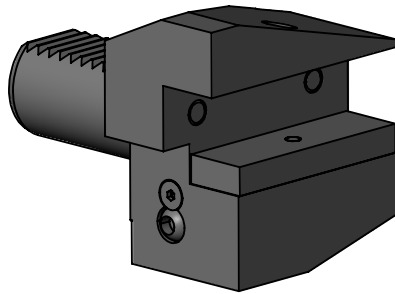
90DEG VDI30 STATIC TOOL OUTPUT: 20mm SQR SHANK COOLANT: EXTERNAL
